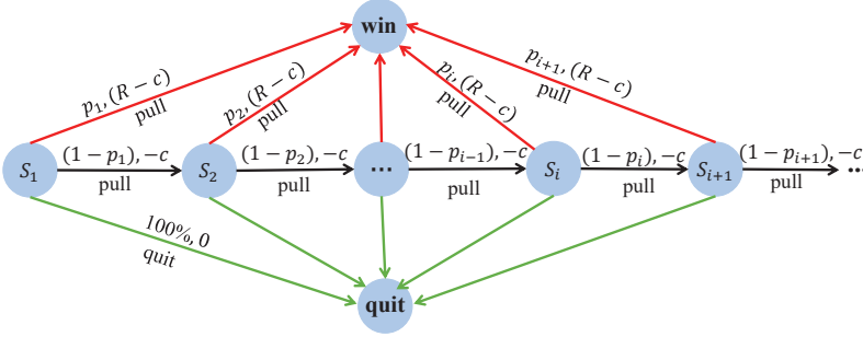
Fig. 1. Markov Decision Process in Gacha Game
